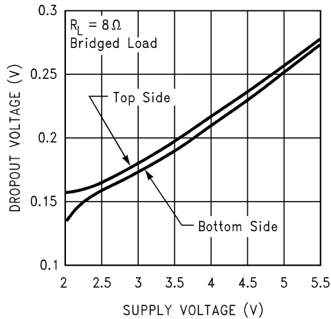
Dropout Voltage
