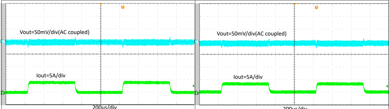
Figure 8-16. TPS564242 Transient Response with 0.1 A to 4 A by 2.5-A/ \mu\text{s} Load Step
