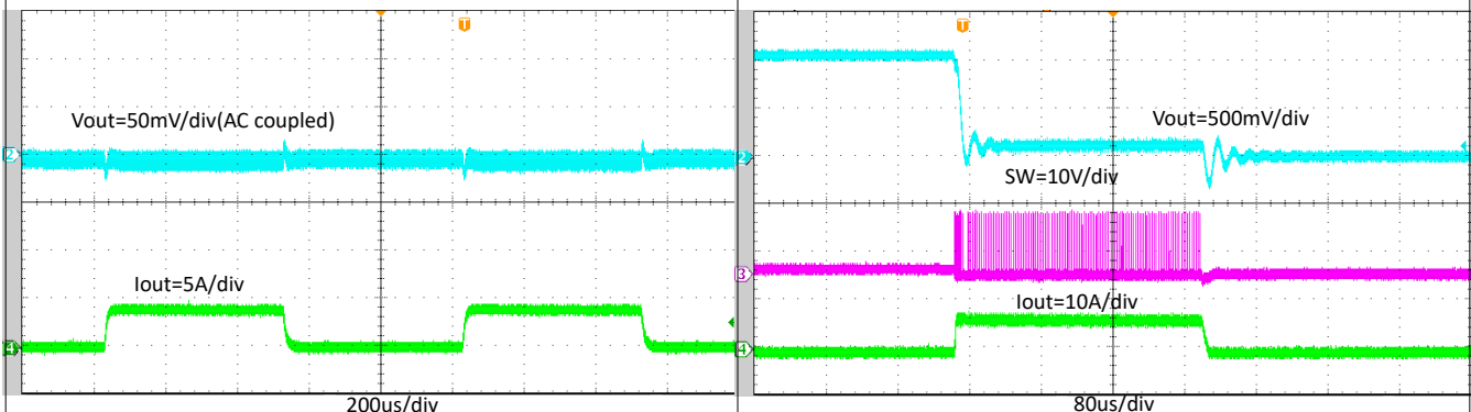
Figure 8-18. TPS564247 Transient Response with 0.1 A to 4 A by 2.5-A/ \mu\text{s} Load Step
