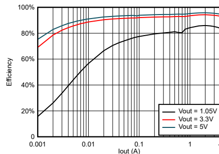
TPS564242 Efficiency at V_{\text{IN}} = 12\text{ V}
