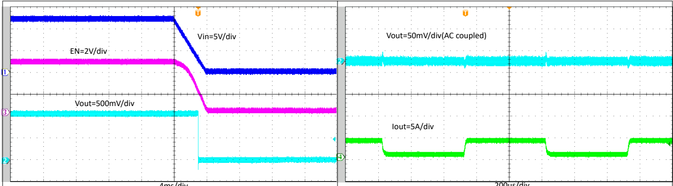
Figure 8-14. Start-Up with V_{IN} Falling, I_{OUT} = 4\text{ A}
