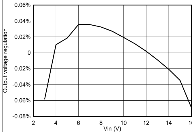
Figure 8-6. TPS564242 Line Regulation vs V_{IN} with 4-A Loading
