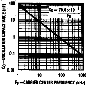
FIGURE 6. Find C_O 's value knowing F_O
