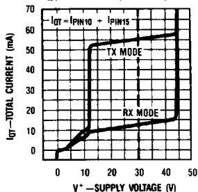
Total Current Consumption, I QT , vs Supply Voltage
