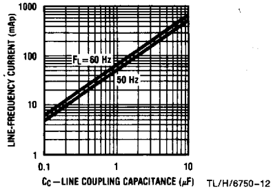
FIGURE 10. The AC line-induced current passed by C C
