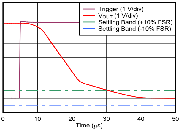
Full scale to zero scale swing Figure 6-22. Voltage Output Setting Time: Falling Edge
