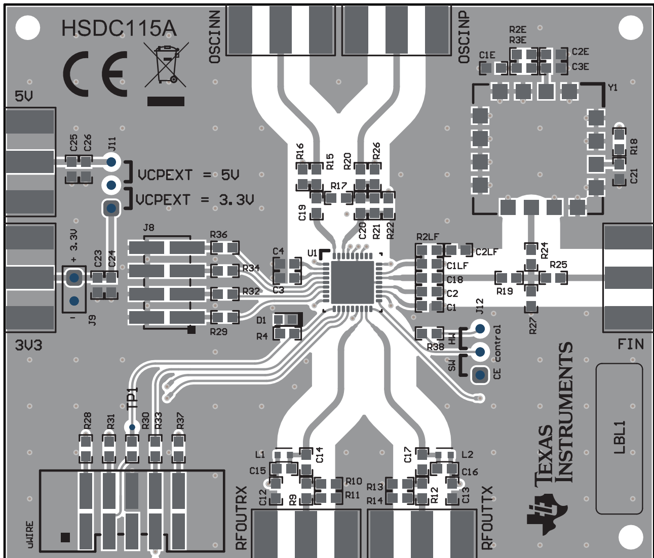
Figure 10-1. Layout Example
