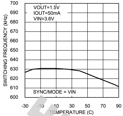
Switching Frequency vs Temperature (PWM Mode)
