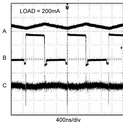
PWM Mode Switching Waveform
