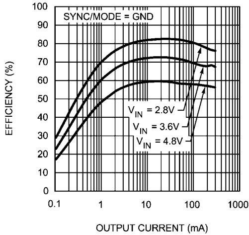
Efficiency vs Output Current ( V_{OUT} = 1.8V , PFM Mode, No Diode)
