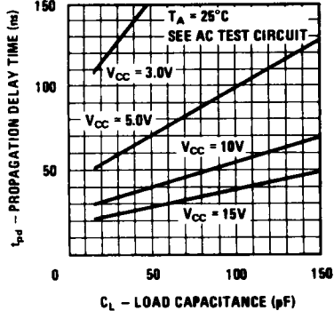
Propagation Delay Time vs Load Capacitance MM54C20/MM74C20
