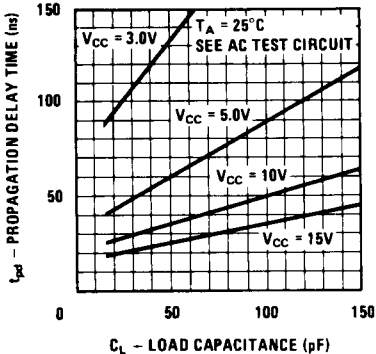
Propagation Delay Time vs Load Capacitance MM54C10/MM74C10
