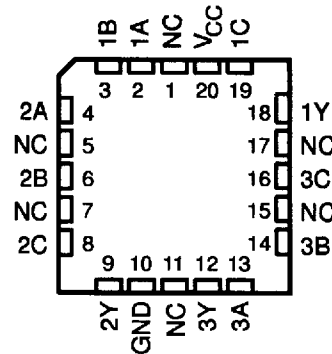
SN54ALS27A, SN54AS27 ... FK PACKAGE (TOP VIEW)
