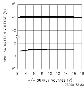
Common-Mode Input Saturation Voltage
