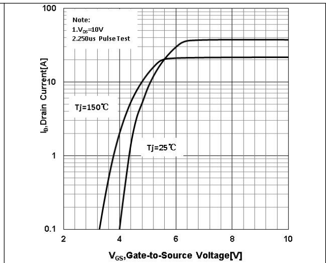
Figure 8. Transfer Characteristics Variation with Source Current
