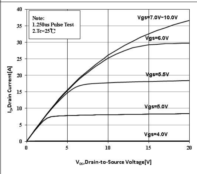
Figure 6. On-State Characteristics
