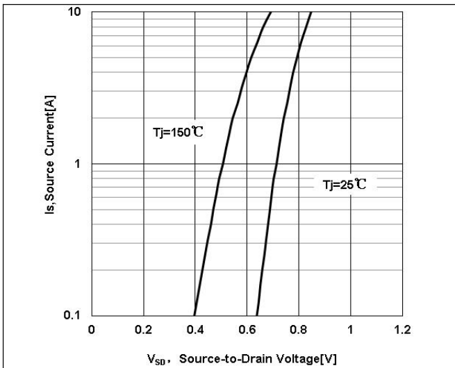
Figure 7. Body Diode Forward Voltage Variation with Source Current
