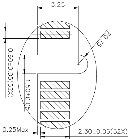
DETAIL A SCALE 12:1
