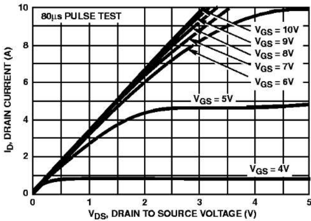
FIGURE 6. SATURATION CHARACTERISTICS
