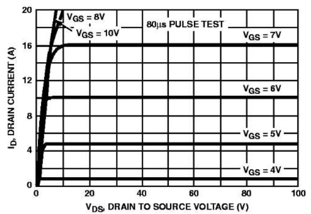
FIGURE 5. OUTPUT CHARACTERISTICS
