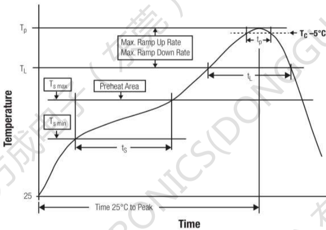
Package Classification Reflow Temperature ( T_c ):
