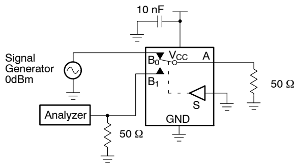
Figure 17. Crosstalk
