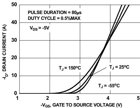
Figure 5. Transfer Characteristics
