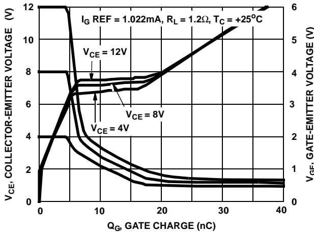
FIGURE 13. GATE CHARGE
