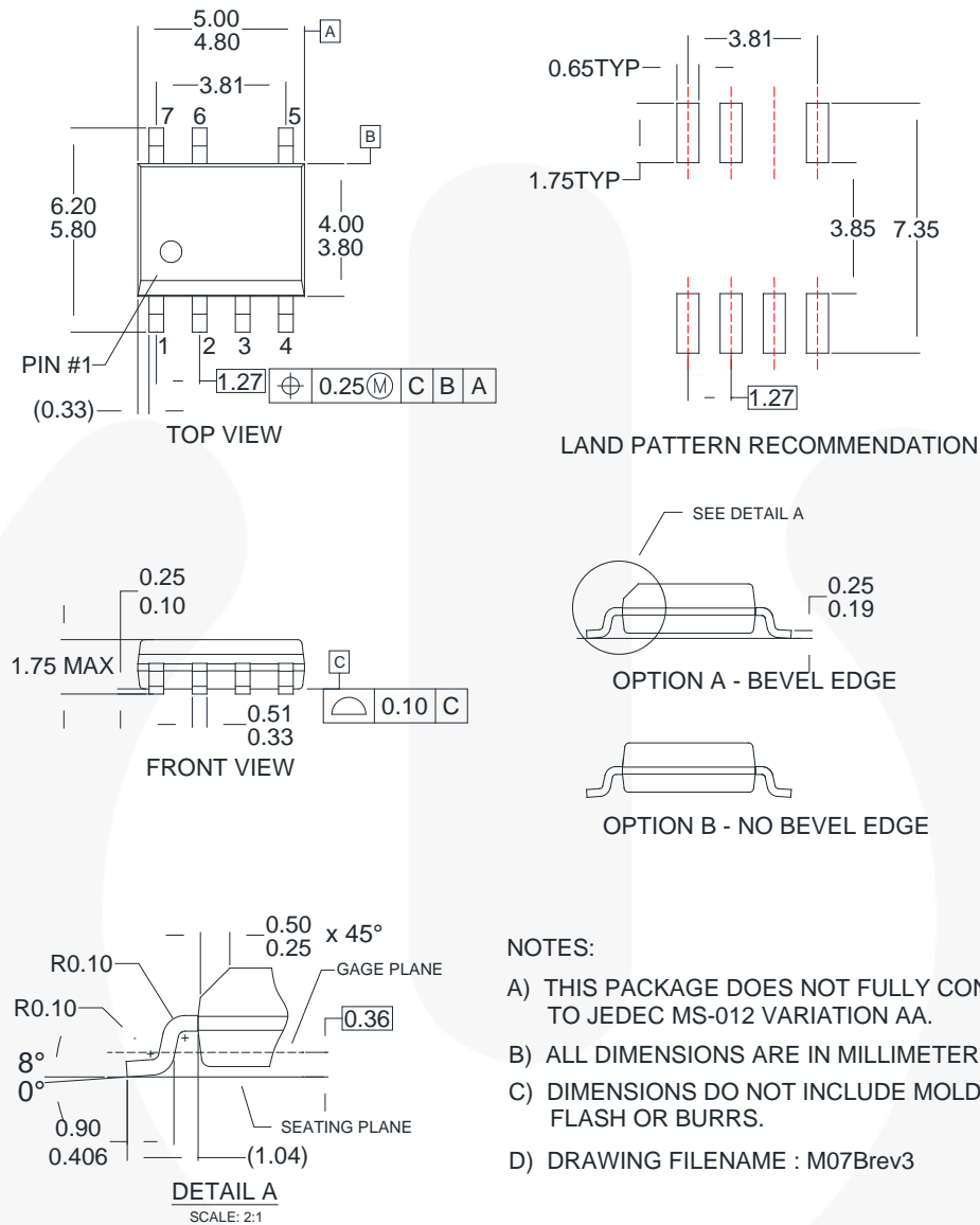
Figure 34. 7-Lead, Small Outline Package (SOP-7)
