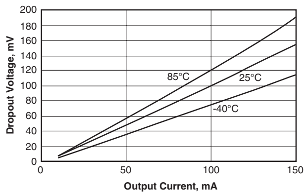
Dropout Voltage vs. I OUT
