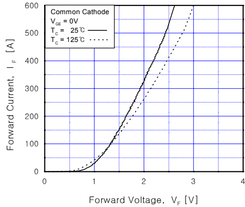
Fig 12. Forward Characteristics(diode)
