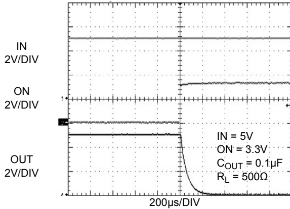
Figure 25. t OFF Response
