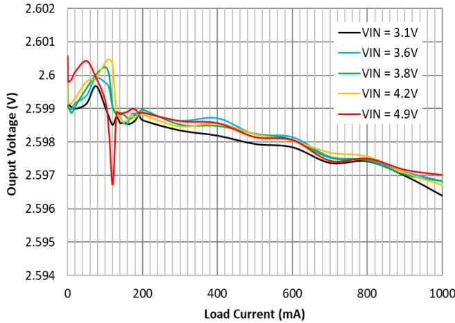
Figure 18. Load Regulation and Input Voltage
