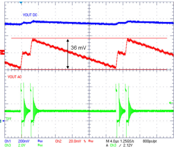
Figure 25. PFM Ripple
