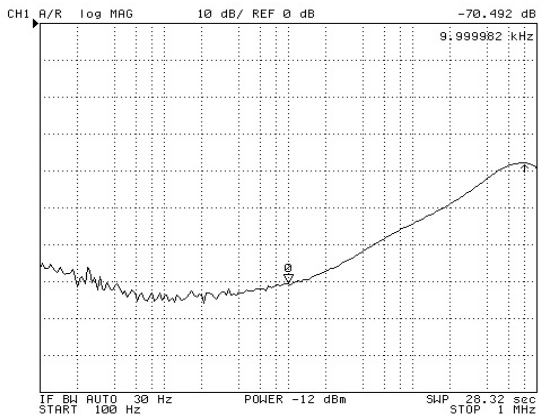
Figure 12. LDO3/4 PSRR vs. Frequency, 50 mA Load
