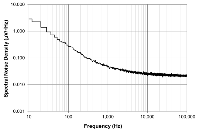
Figure 17. LDO5 Output Noise vs. Frequency, 300 mA Load
