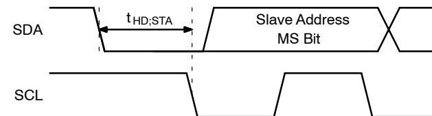
Figure 24. Start Bit
