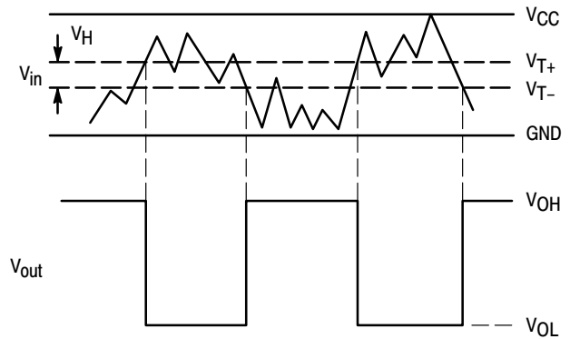
Figure 5. Typical Schmitt-Trigger Applications
