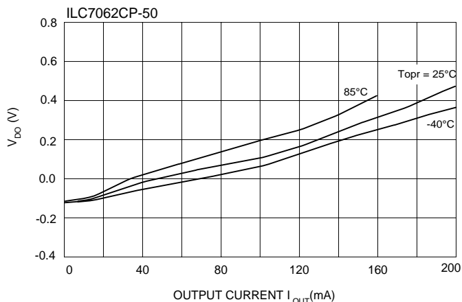
V DD vs Output Current
