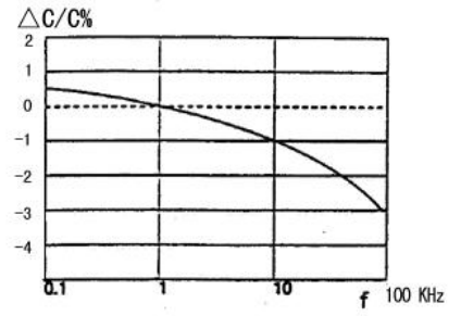
Capacitance vs. frequency (Room temperature)
