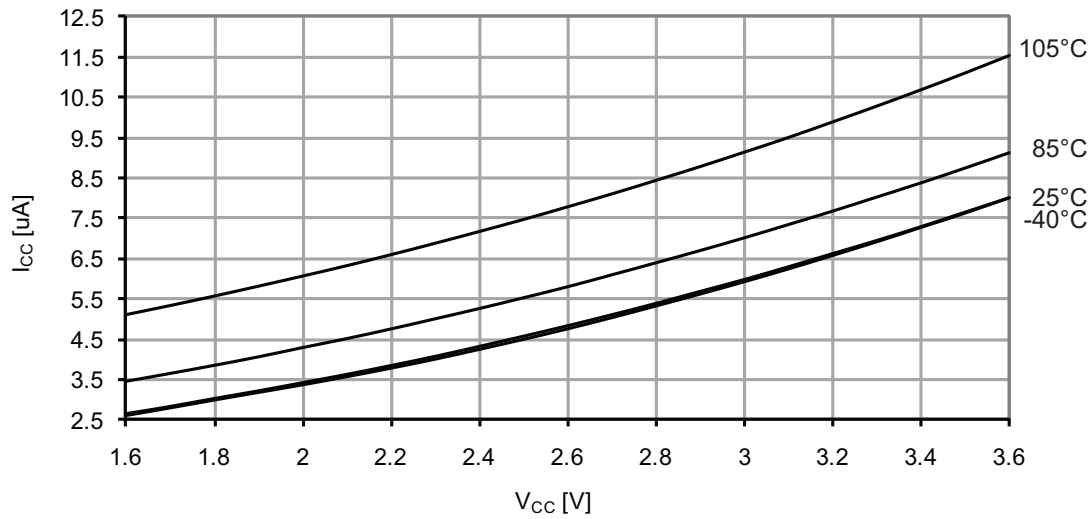
Figure 37-184. Standby supply current vs. V_{CC} . Standby, f_{SYS} = 1\text{MHz} .
