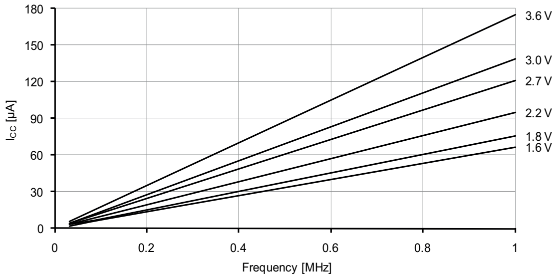
Figure 37-91. Idle mode supply current vs. frequency.
