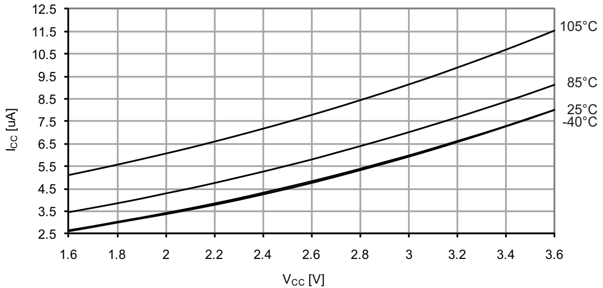
Figure 37-18. Standby supply current vs. V_{CC} . Standby, f_{SYS} = 1\text{MHz} .
