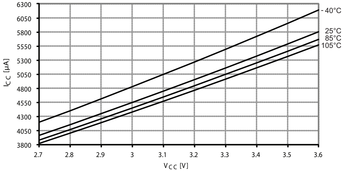
Figure 37-14. Idle mode current vs. V_{CC} . f_{SYS} = 32MHz internal oscillator.
