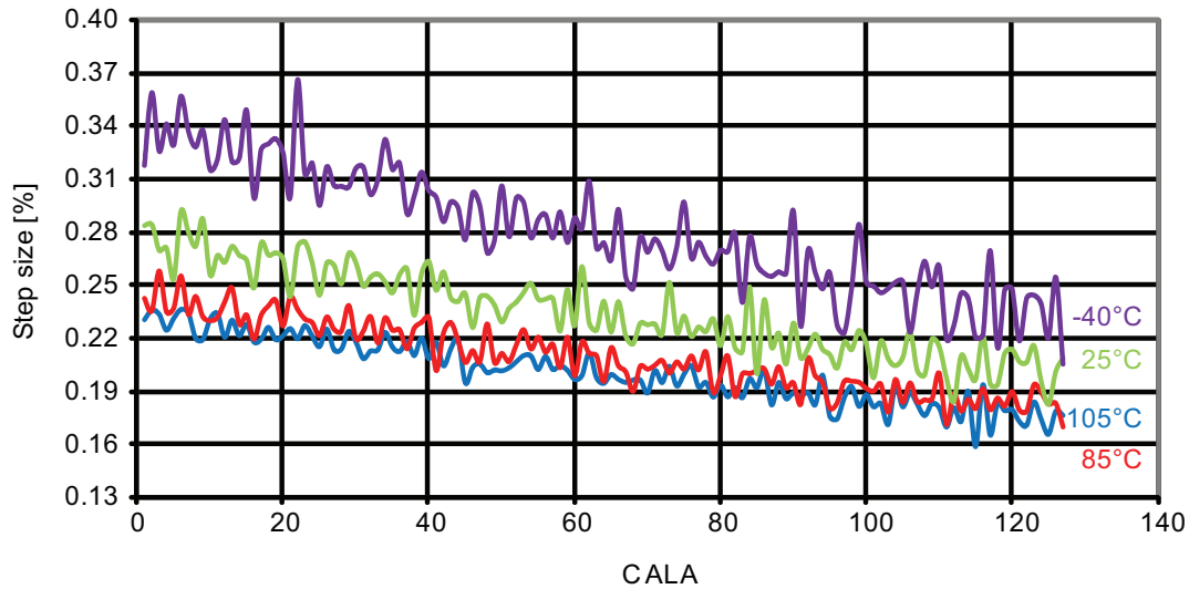
Figure 37-322. 2MHz internal oscillator CALA calibration step size.
