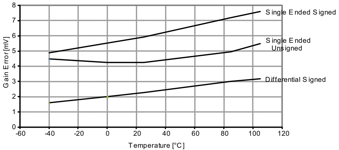
Figure 37-44. Gain error vs. temperature. V_{CC} = 2.7\text{V} , V_{REF} = \text{external } 1.0\text{V} .
