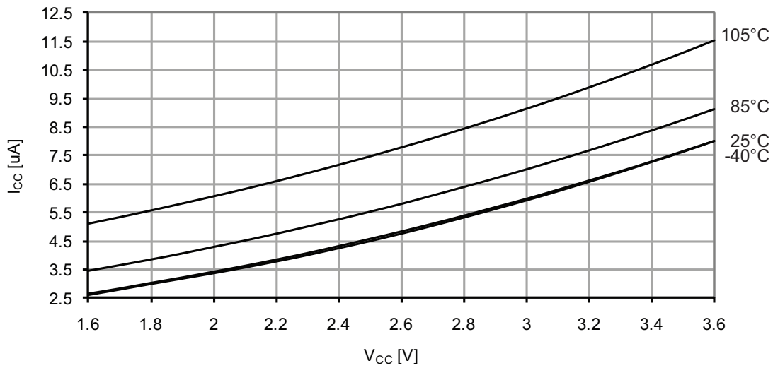
Figure 37-267. Standby supply current vs. V_{CC} . Standby, f_{SYS} = 1\text{MHz} .
