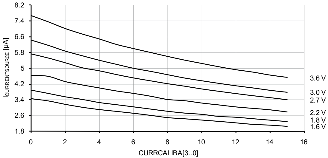
Figure 37-139. Analog comparator current source vs. calibration value.
