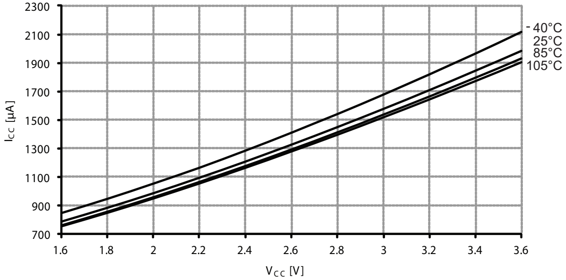
Figure 37-13. Idle mode supply current vs. V_{CC} . f_{SYS} = 32MHz internal oscillator prescaled to 8MHz.
