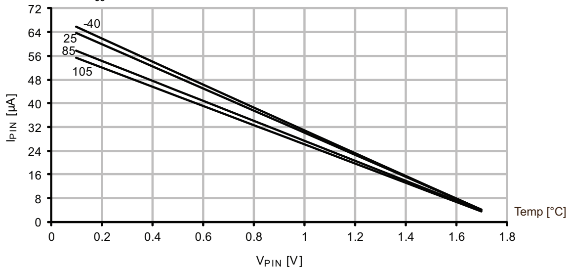
Figure 37-103. I/O pin pull-up resistor current vs. input voltage.
