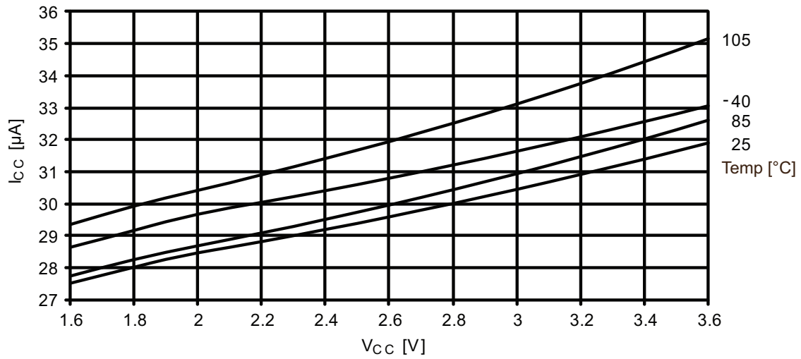
Figure 37-93. Idle mode supply current vs. V_{CC} .
