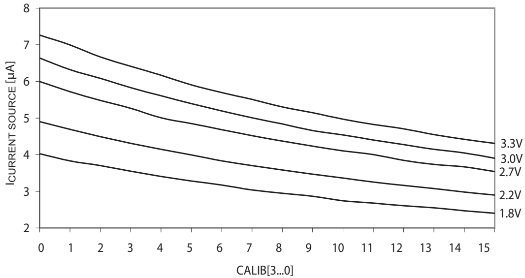
Figure 37-222. Analog comparator current source vs. calibration value.
