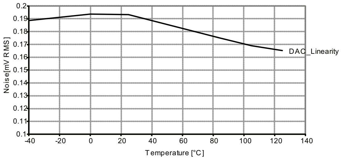
Figure 37-299. DAC noise vs. temperature.
