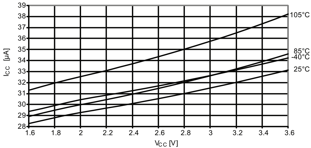
Figure 37-176. Idle mode supply current vs. V_{CC} .
