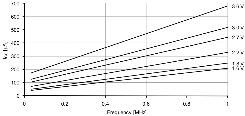
Figure 37-1. Active supply current vs. frequency. f_{SYS} = 0 - 1MHz external clock, T = 25^{\circ}C .
