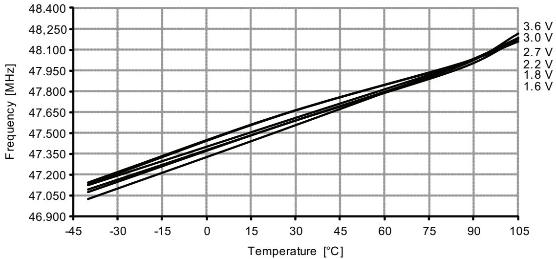
Figure 37-79. 48MHz internal oscillator frequency vs. temperature. DPLL enabled, from the 32.768kHz internal oscillator.
