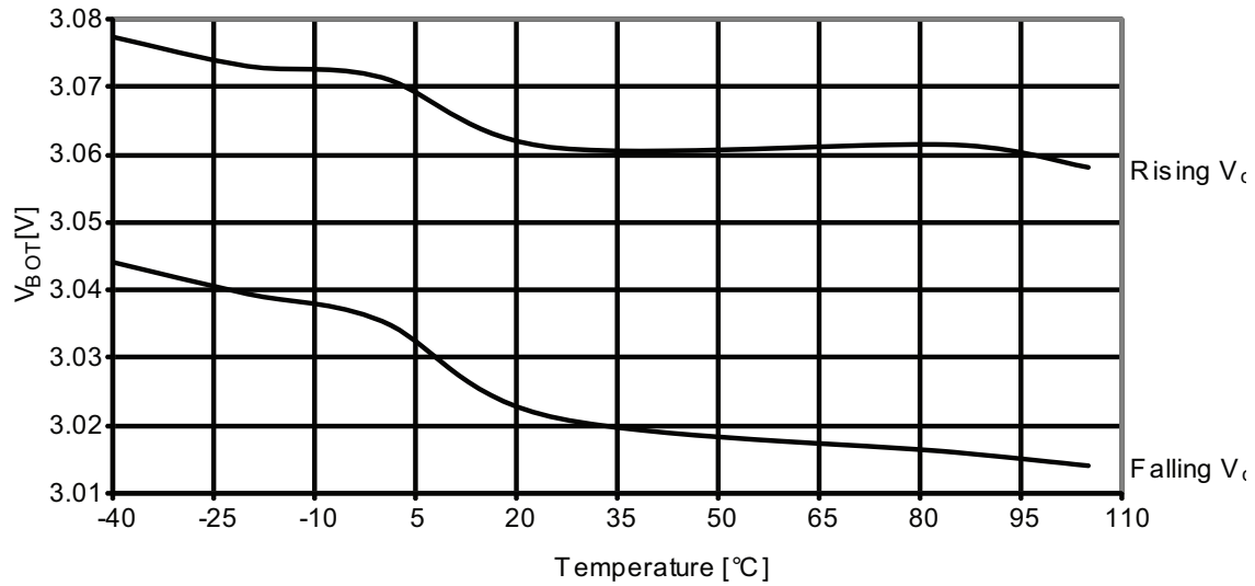
Figure 37-309. BOD thresholds vs. temperature.
