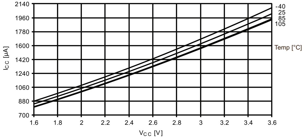
Figure 37-96. Idle mode supply current vs. V_{CC} . f_{SYS} = 32MHz internal oscillator prescaled to 8MHz.
