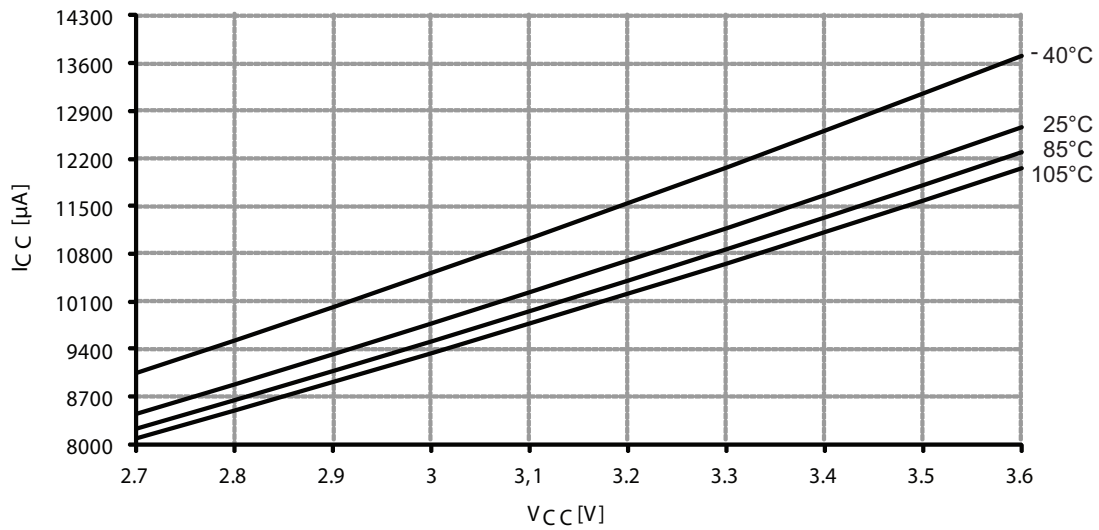
Figure 37-7. Active mode supply current vs. V_{CC} .
