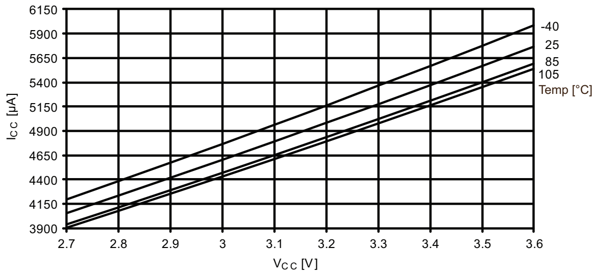
Figure 37-97. Idle mode current vs. V_{CC} . f_{SYS} = 32MHz internal oscillator.
