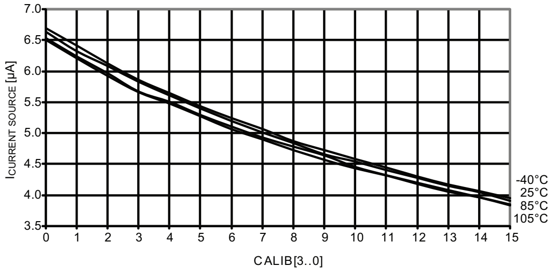
Figure 37-222. Analog comparator current source vs. calibration value.
