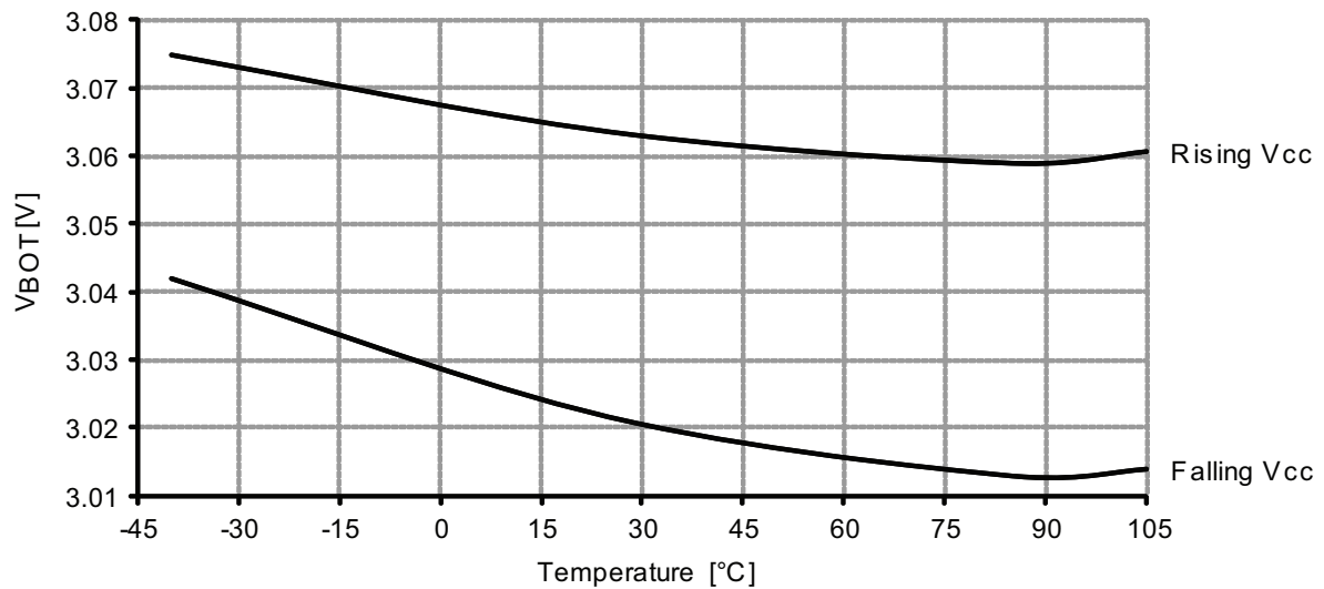
Figure 37-60. BOD thresholds vs. temperature.
