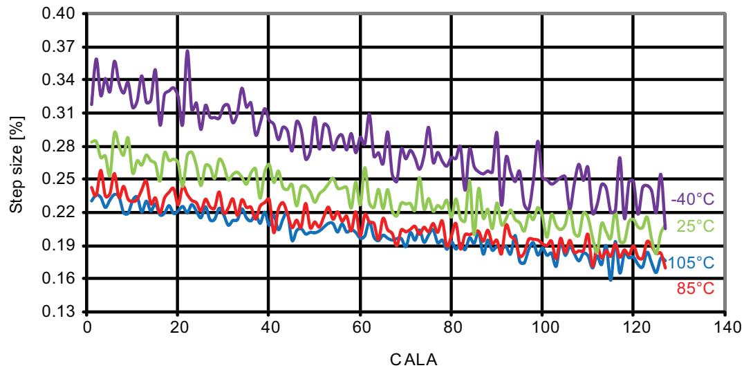
Figure 37-239. 2MHz internal oscillator CALA calibration step size.
