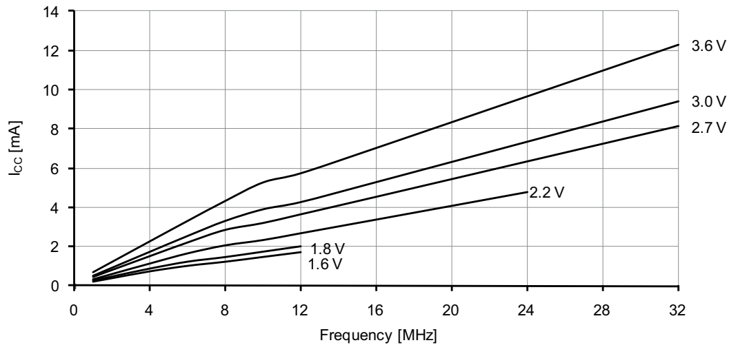
Figure 37-2. Active supply current vs. frequency. f_{SYS} = 1 - 32MHz external clock, T = 25^{\circ}C .
