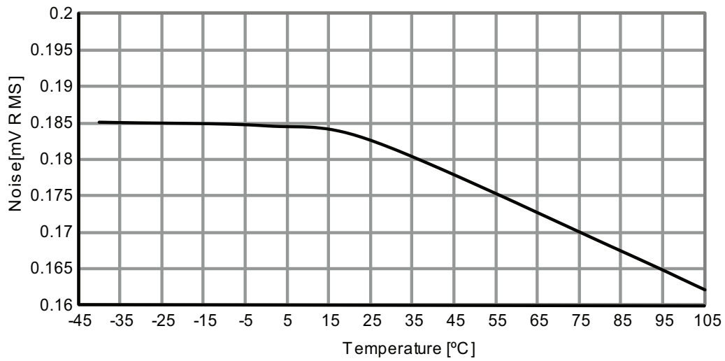
Figure 37-133. DAC noise vs. temperature.
