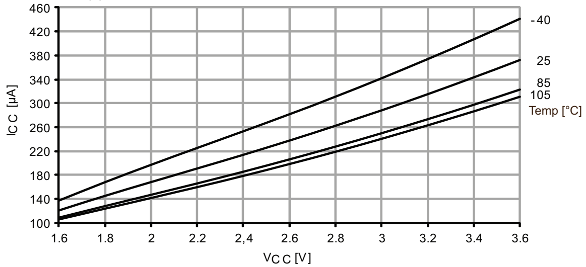
Figure 37-87. Active mode supply current vs. V_{CC} .
