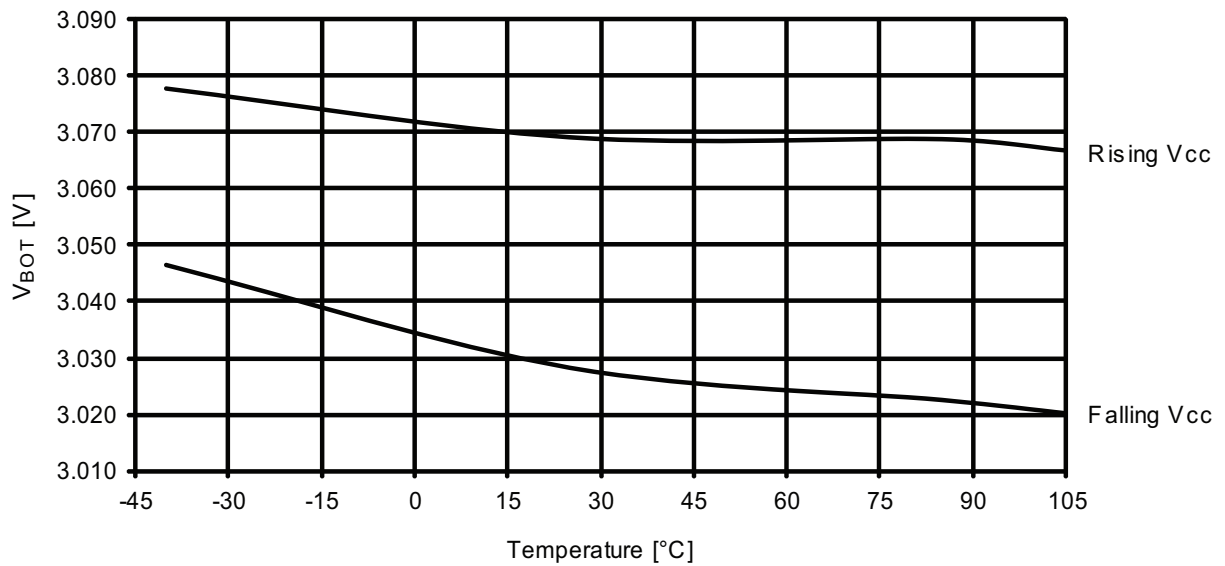
Figure 37-143. BOD thresholds vs. temperature.
