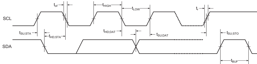
Figure 36-28. Two-wire interface bus timing.
