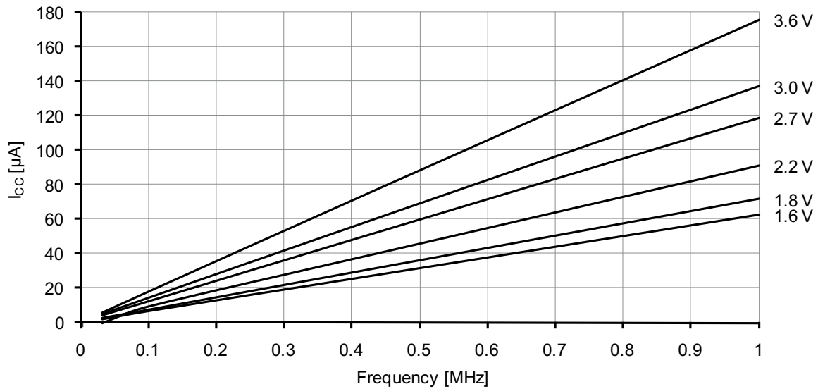
Figure 37-8. Idle mode supply current vs. frequency.
