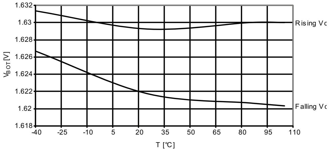
Figure 37-309. BOD thresholds vs. temperature.
