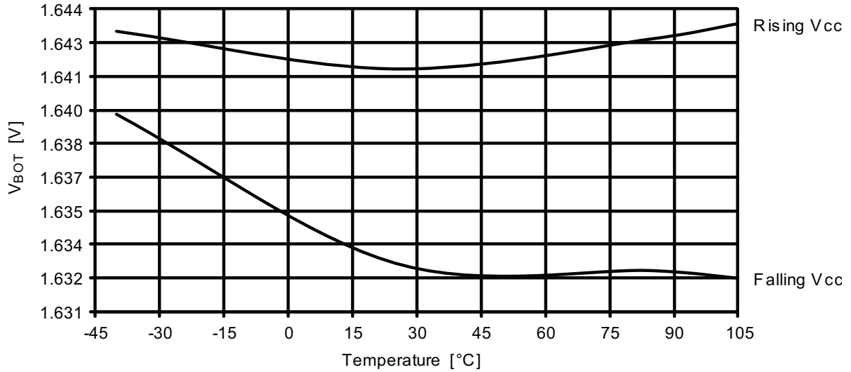
Figure 37-143. BOD thresholds vs. temperature.
