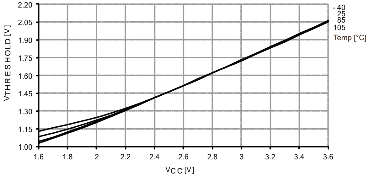
Figure 37-66. Reset pin input threshold voltage vs. V_{CC} .
