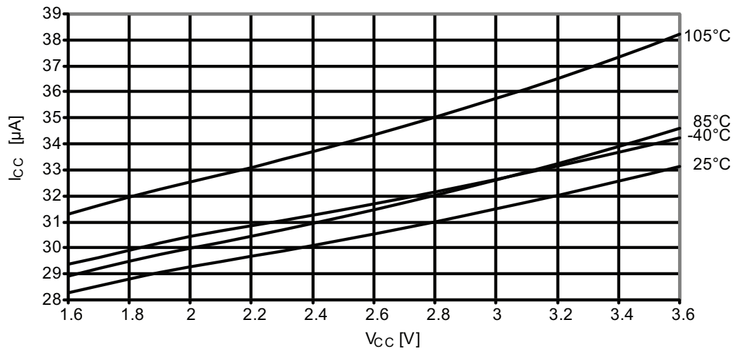
Figure 37-259. Idle mode supply current vs. V_{CC} .
