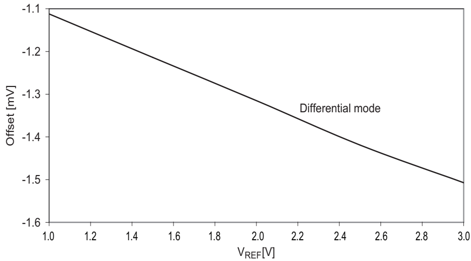
Figure 37-292. Offset error vs. V_{REF} .
