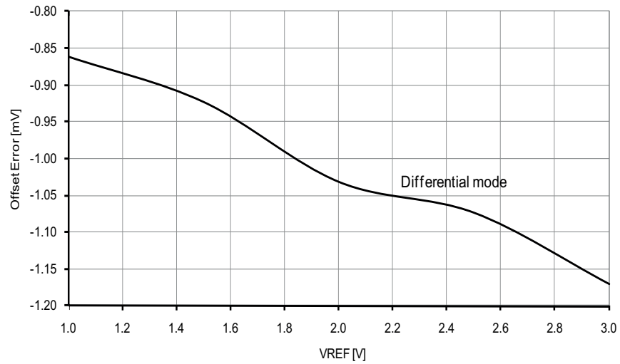
Figure 37-43. Offset error vs. V_{REF} . T = 25^{\circ}\text{C} , V_{CC} = 3.6\text{V} , ADC sampling speed = 500kpsps.
