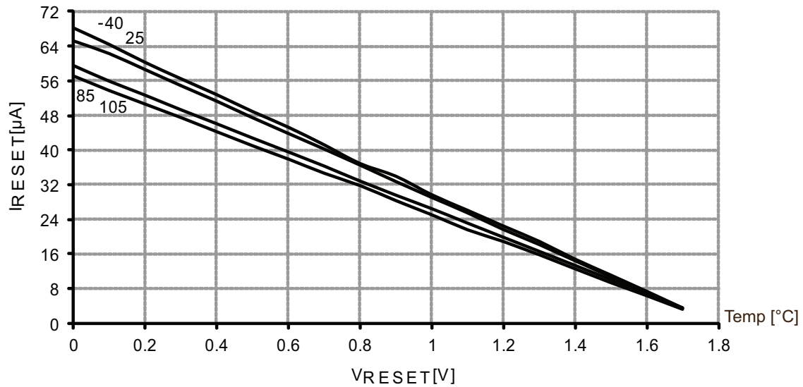
Figure 37-62. Reset pin pull-up resistor current vs. reset pin voltage.
