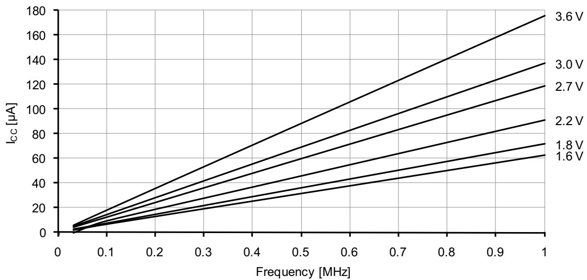
Figure 37-8. Idle mode supply current vs. frequency.
