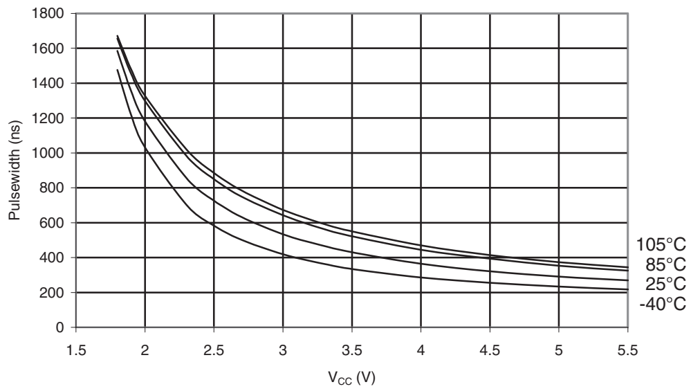
Figure 31-284. ATmega168PA: Minimum Reset Pulse Width vs. V CC
