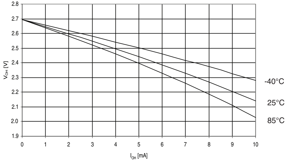
Figure 31-147. Atmel ATmega329A: I/O pin output voltage vs. source current, ports A, C, D, E, F, G ( V_{CC} = 2.7V ).
