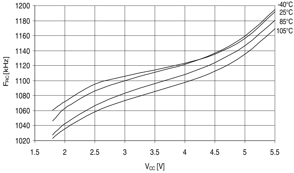
Figure 32-281. ATmega3290A - 105°C: Watchdog Oscillator Frequency vs. V_{CC}
