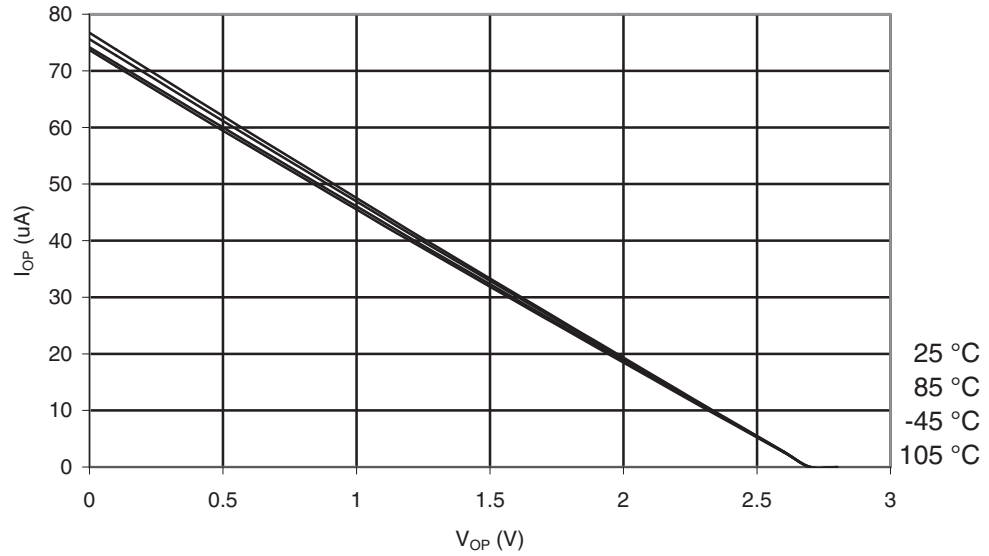
Figure 32-16. ATmega169PA-105°C: I/O Pin Pull-up Resistor Current vs. Input Voltage ( V_{CC} = 2.7V )
