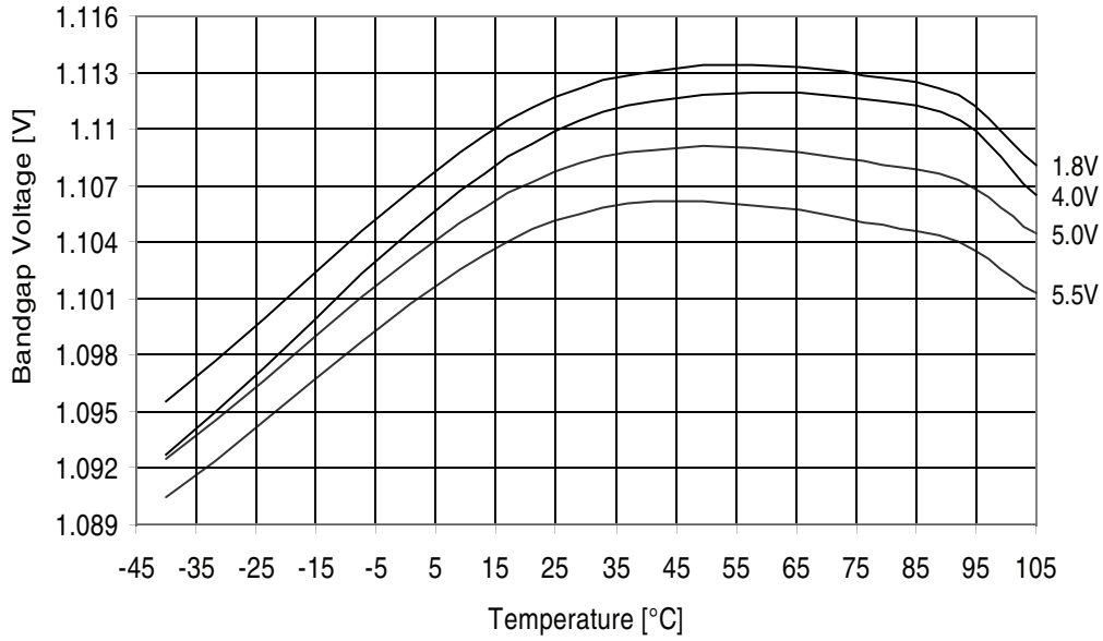
Figure 32-216. ATmega329PA - 105°C: Bandgap Voltage vs. Temperature
