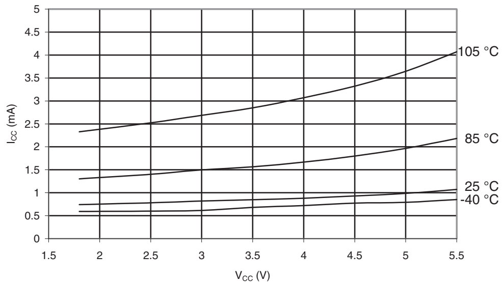
Figure 32-313. ATmega3290PA-105°C: Standby Supply Current vs. V_{CC} (32kHz Watch Crystal, Watchdog Timer Disabled)
