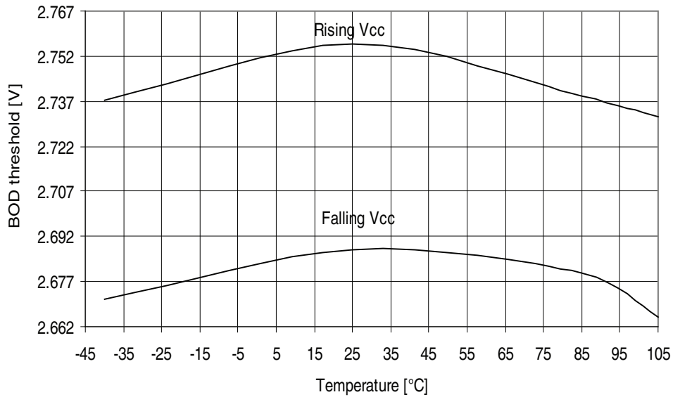
Figure 32-276. ATmega3290A - 105°C: BOD Thresholds vs. Temperature (BOD Level is 2.7V)
