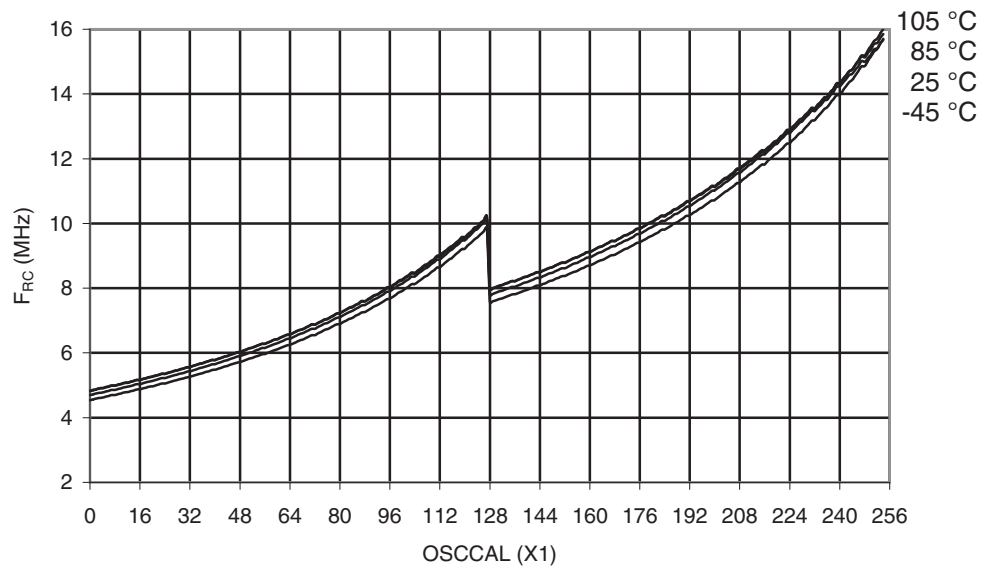
Figure 32-47. ATmega169PA-105°C: Calibrated 8MHz RC Oscillator Frequency vs. OSCCAL Value
