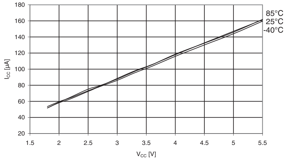
Figure 31-298. ATmega3290A: AREF external reference current vs. V_{CC} .
