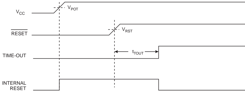
Figure 11-3. MCU Start-up, RESET Extended Externally
