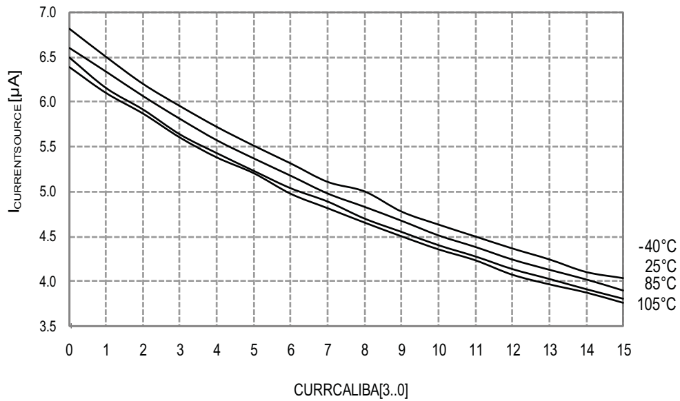
Figure 34-115. Analog Comparator Current Source vs. Calibration Value
