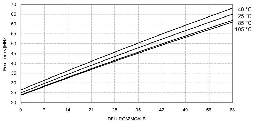
Figure 34-207. 32MHz Internal Oscillator Frequency vs. CALB Calibration Value
