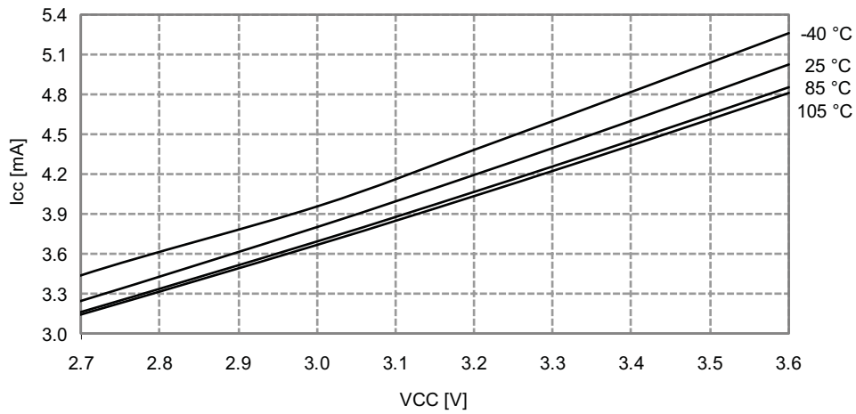
Figure 34-226. Idle Mode Current vs. V_{CC} f_{SYS} = 32\text{MHz} internal oscillator
