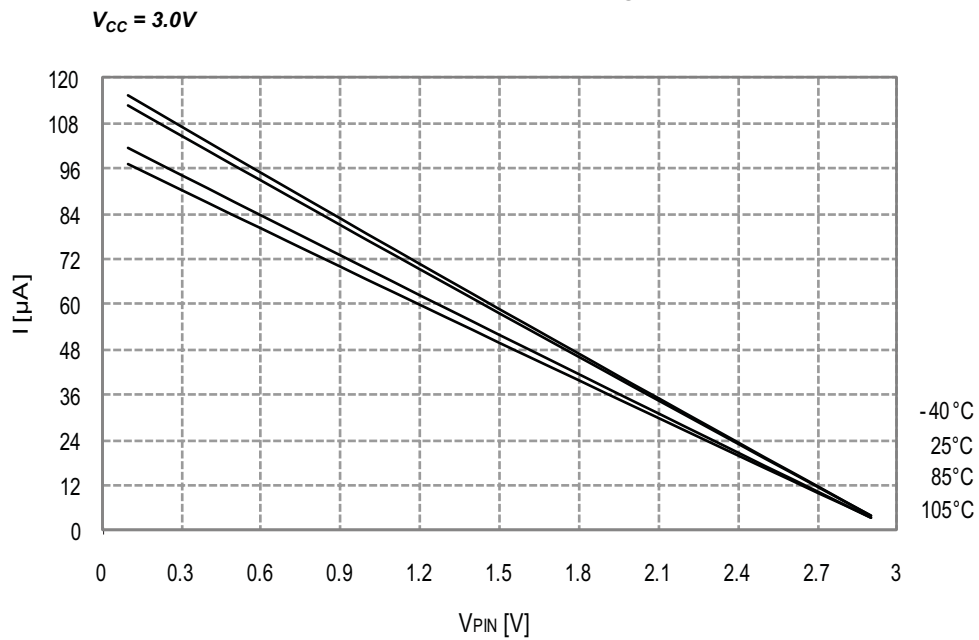
Figure 34-20. I/O Pin Pull-up Resistor Current vs. Input Voltage
