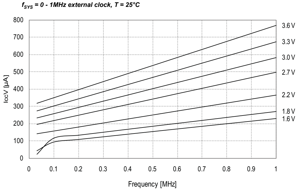
Figure 34-72. Active Supply Current vs. Frequency
