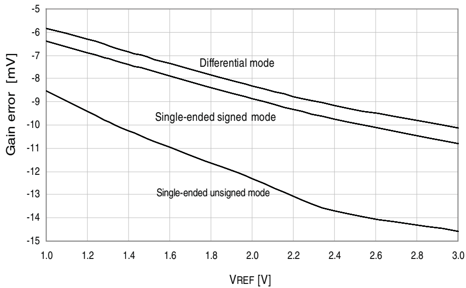
Figure 34-178. Gain Error vs. V_{REF} T = 25^\circ\text{C} , V_{CC} = 3.6\text{V} , ADC sample rate = 300kps
