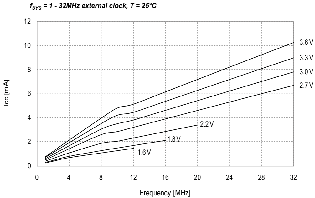
Figure 34-73. Active Supply Current vs. Frequency
