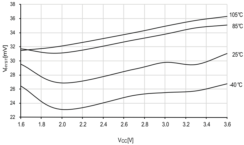
Figure 34-114. Analog Comparator Hysteresis vs. V_{CC}
