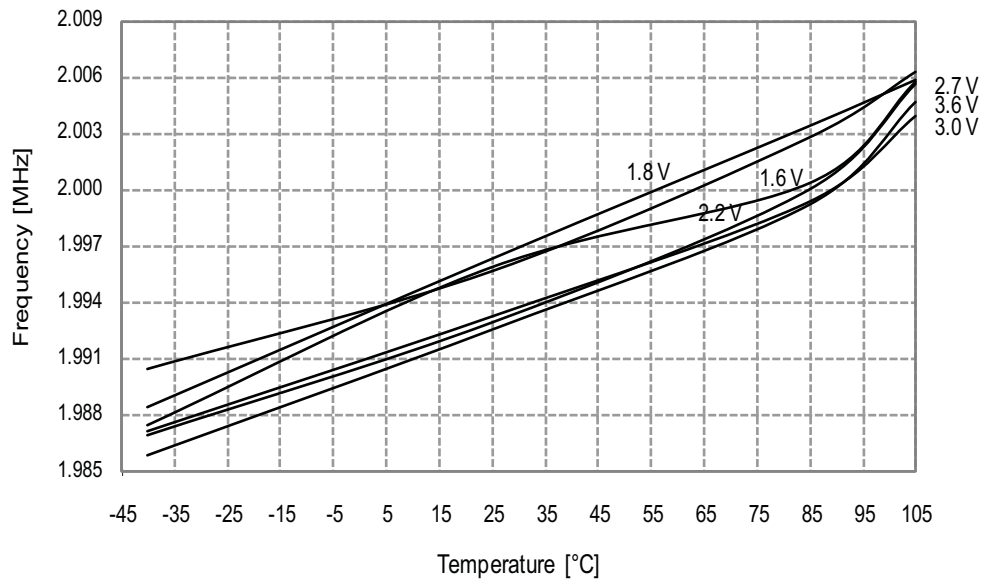
Figure 34-58. 2MHz Internal Oscillator Frequency vs. Temperature DPLL enabled, from the 32.768kHz internal oscillator
