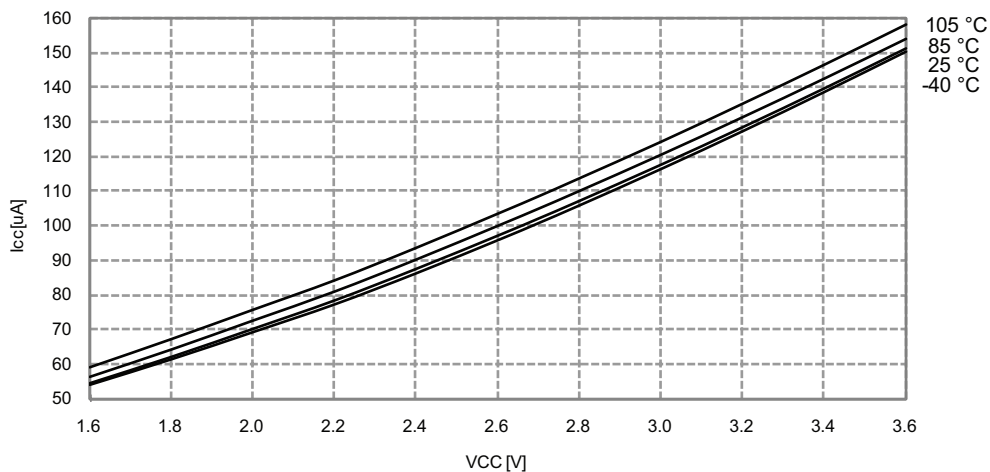
Figure 37-263. Idle mode supply current vs. V_{CC} .
