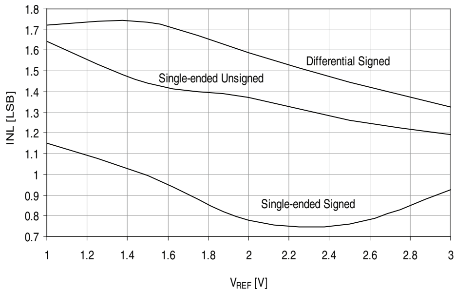
Figure 37-288. INL error vs. external V_{REF}
