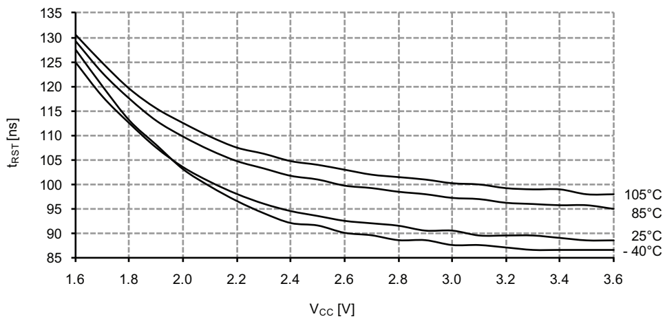
Figure 37-230. Minimum Reset pin pulse width vs. V CC .
