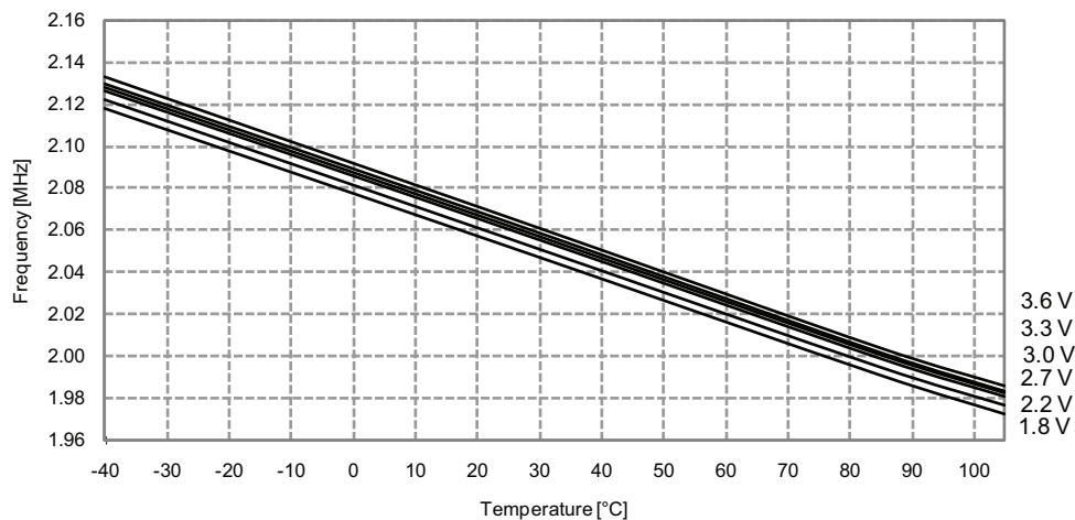
Figure 37-325. 2MHz internal oscillator frequency vs. temperature DPLL disabled
