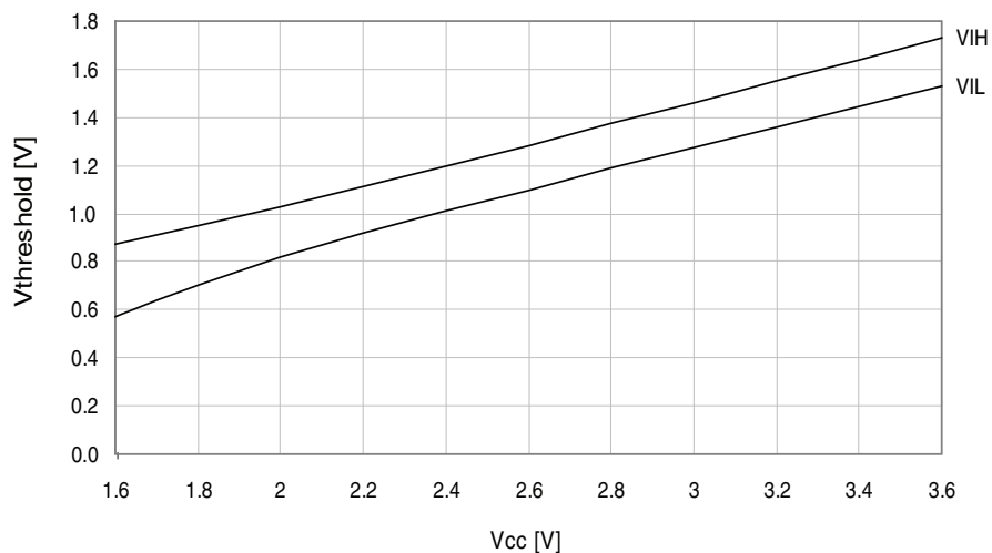
Figure 37-200. I/O pin input threshold voltage vs. V_{CC} .
