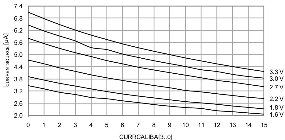
Figure 37-57. Analog comparator current source vs. calibration value.
