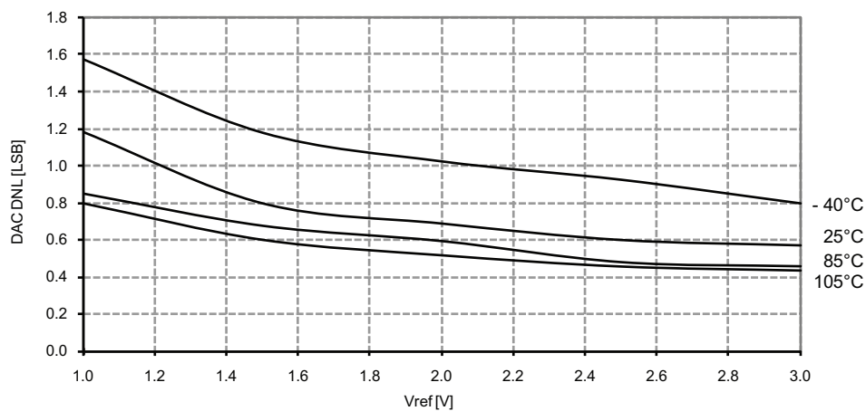
Figure 37-218. DNL error vs. V_{REF} .
