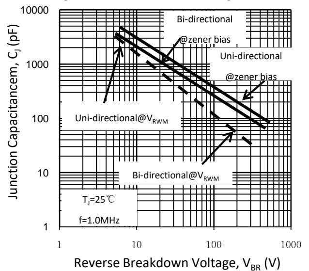
Fig. 6-Typical Junction Capacitance
