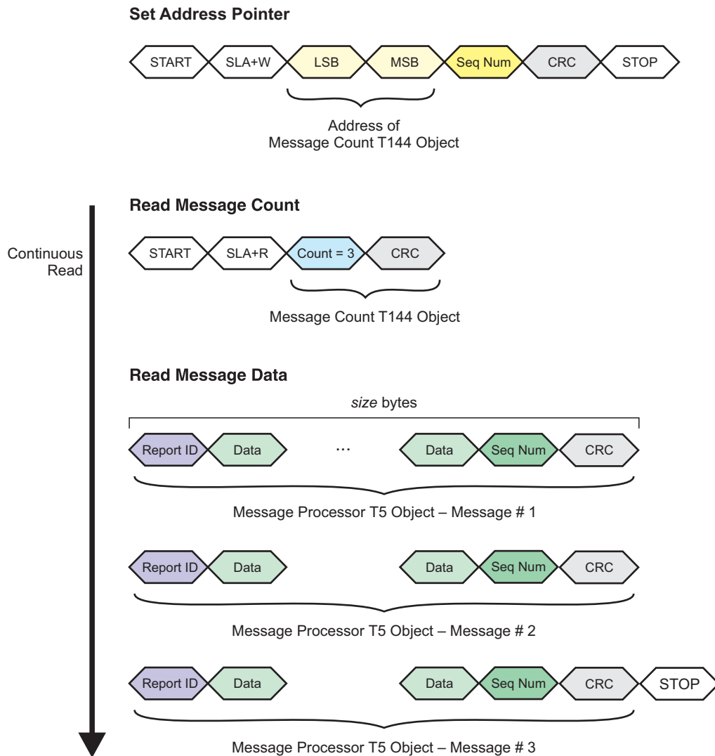
FIGURE 8-4: CONTINUOUS READ EXAMPLE
