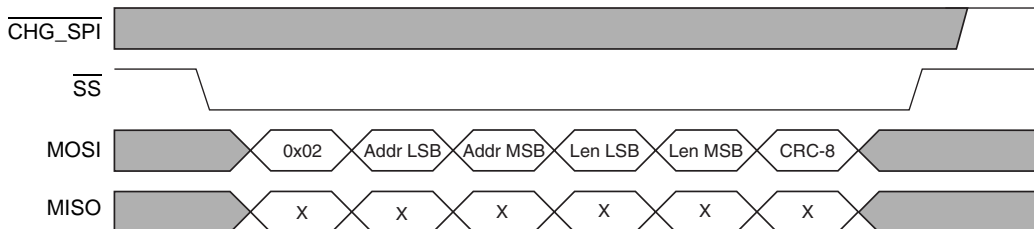
FIGURE 9-6: SPI_READ_REQ
