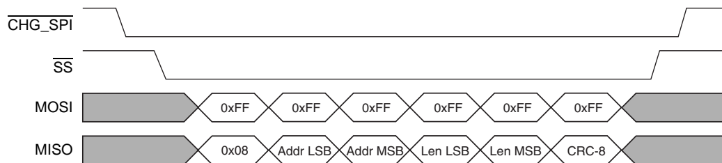
FIGURE 9-11: SPI_INVALID_CRC
