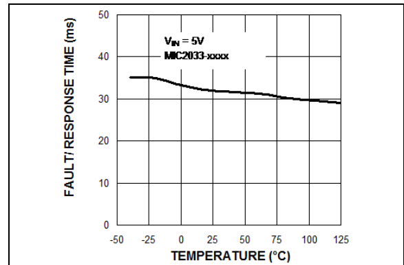
FIGURE 2-17: FAULT/ Response Time vs. Temperature.
