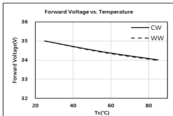
c) Temperature Characteristics ( I_f = Sorting Current)
