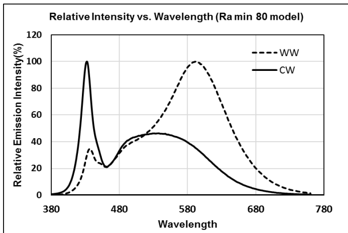
a) Spectrum Distribution ( I_f = Sorting Current, T_j = 25^\circ\text{C} )
