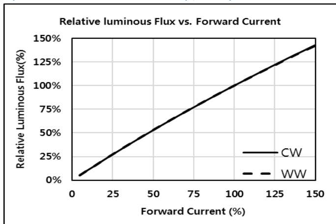
b) Forward Current Characteristics ( T_j = 25^\circ\text{C} )
