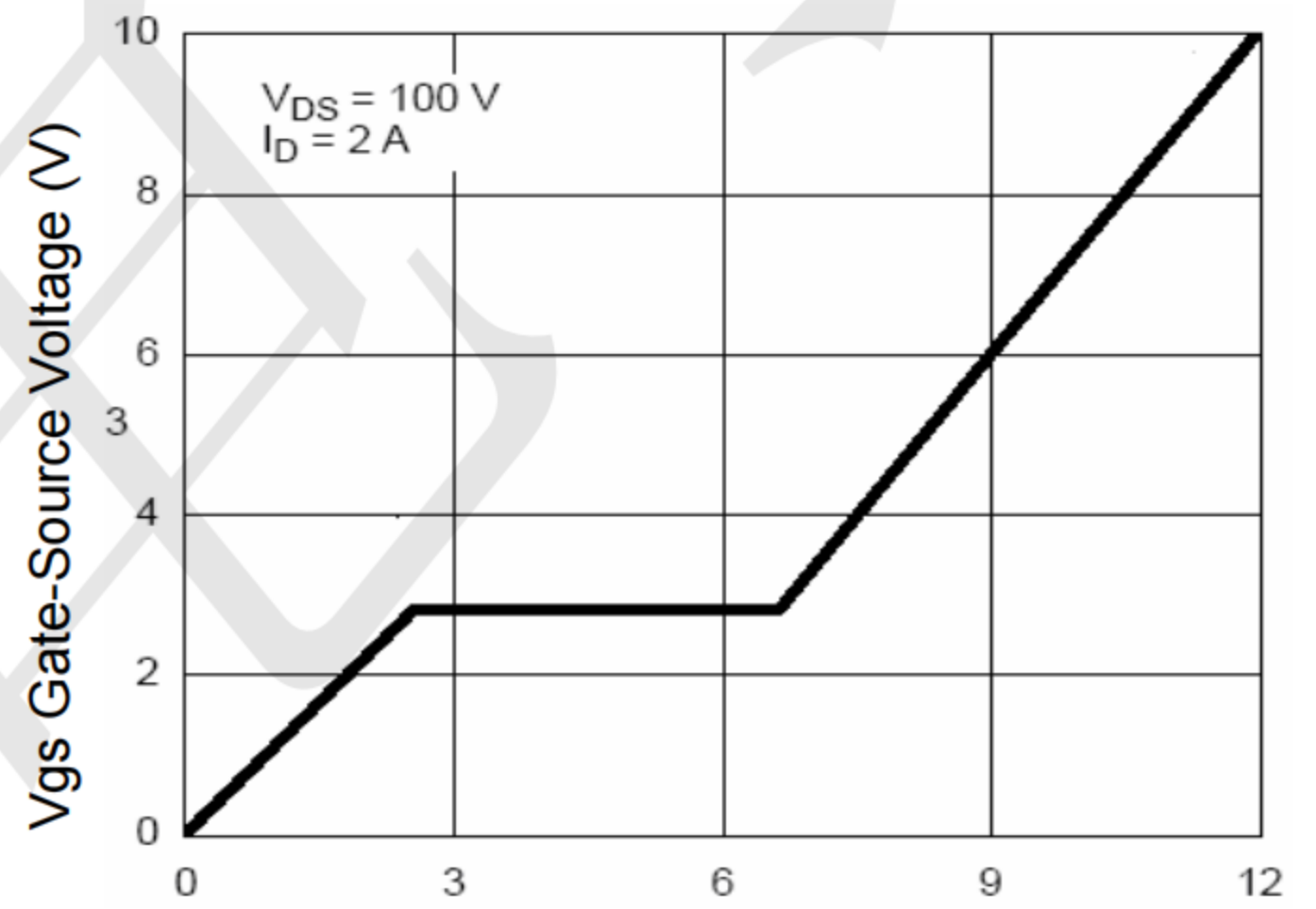
Figure 5 Gate Charge
