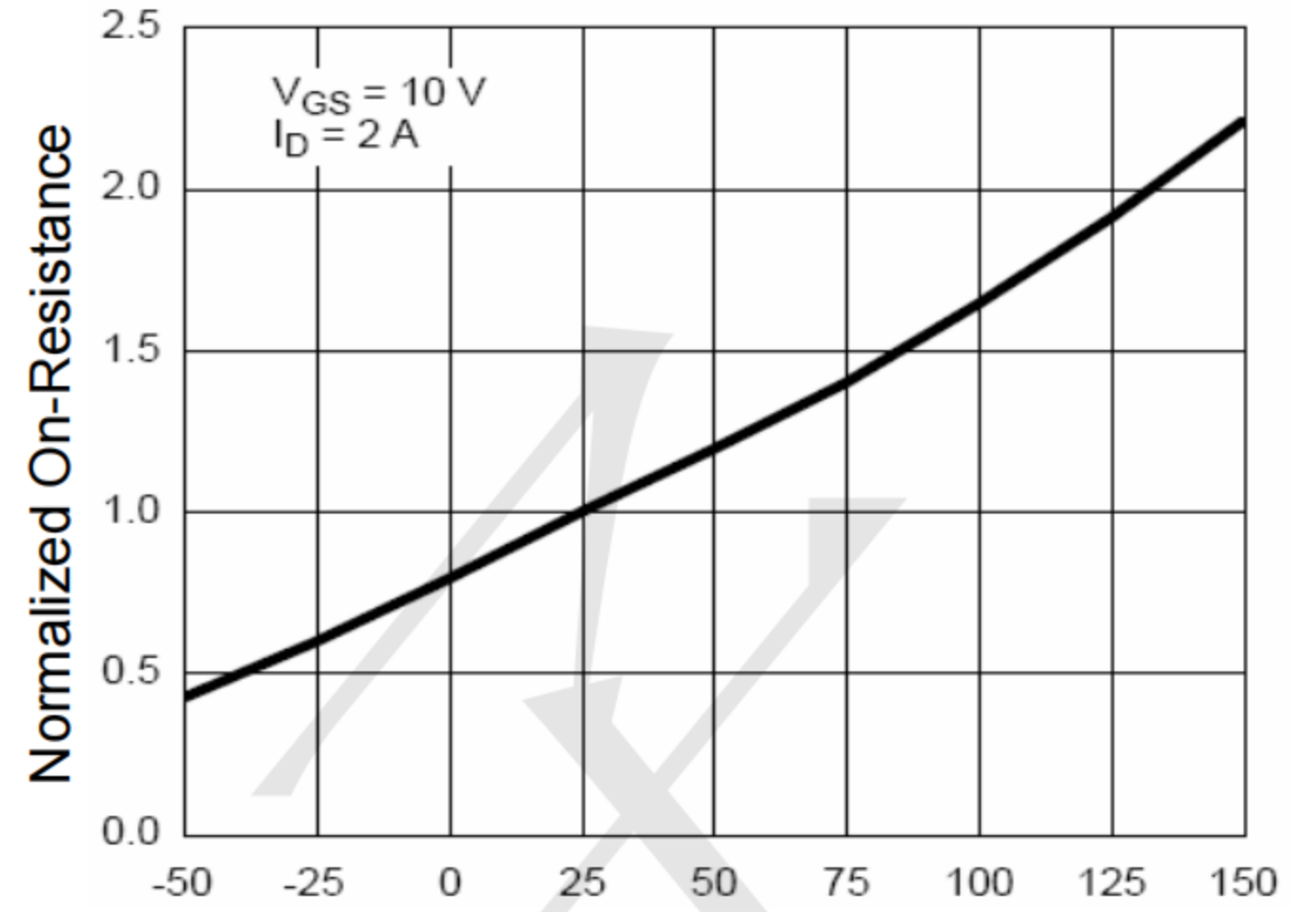
Figure 4 R_{DS(on)} -Junction Temperature
