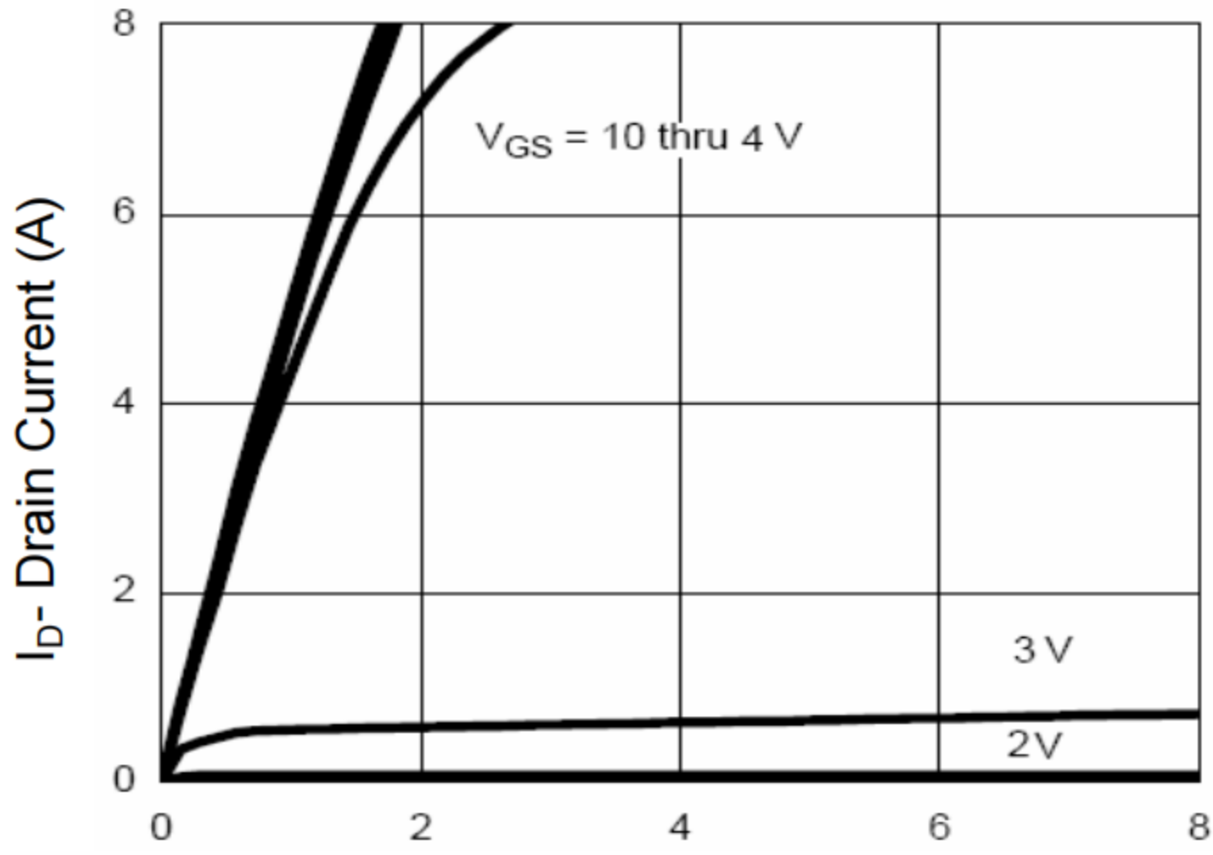
Figure 1 Output Characteristics
