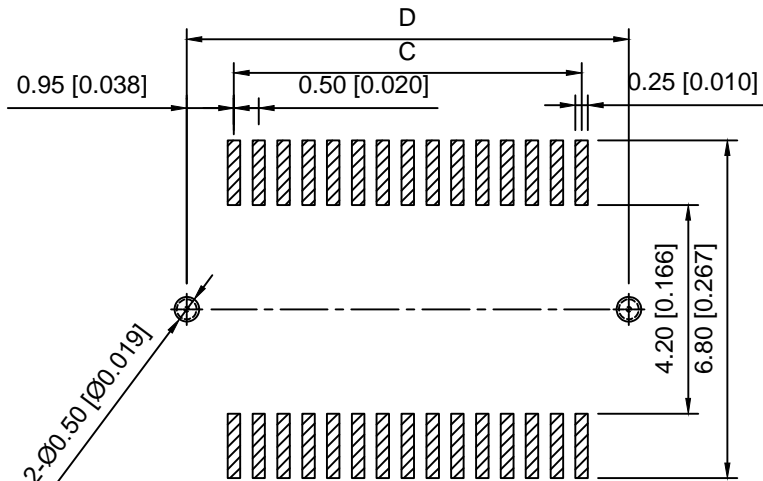
RECOMMENDED PCB PATTERN DIM
