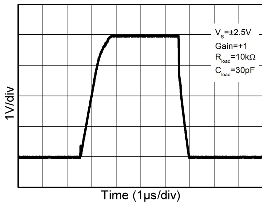
Large-Scale Step Response, 4V Step
