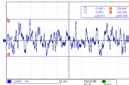
0.1Hz to 10Hz Integrated Input Noise, Gain = 100000
