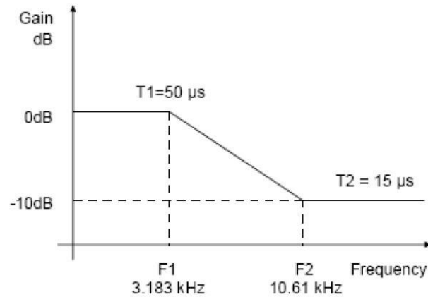
Figure 5. De-Emphasis Curve ( F_s = 44.1 kHz)
