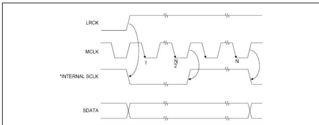
Figure 2. Internal Serial Mode Input Timing
