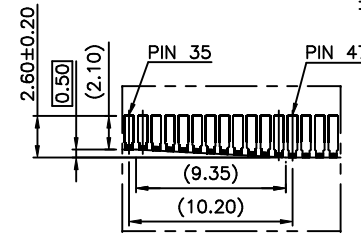
DETAIL E SCALE 2:1
