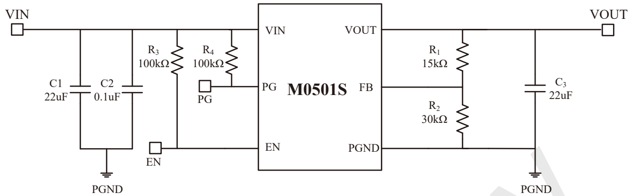
Figure 2. Typical Application Circuits of M0501S for 1.2V@1.5A Output
