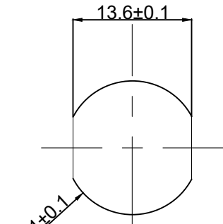
Panel hole size (面板开孔尺寸)
