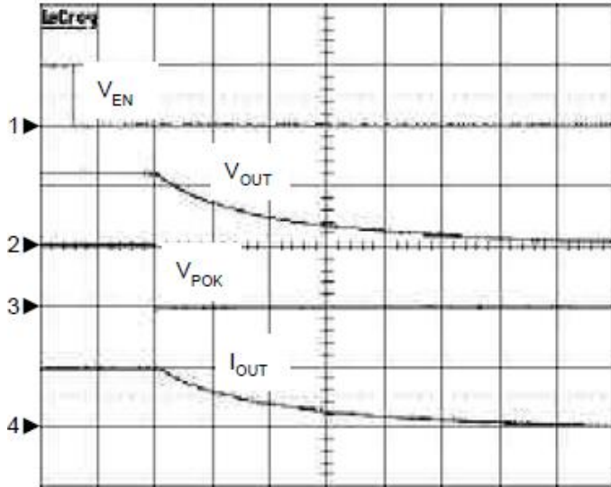
COUT=10mF, CIN=10mF, RL=0.6W/ TIME: 5us/Div CH1: VEN, 5V/Div, DC/CH2: VOUT, 1V/Div, DC CH3: VPOK, 5V/Div, DC/CH4: IOUT, 3A/Div, DC
