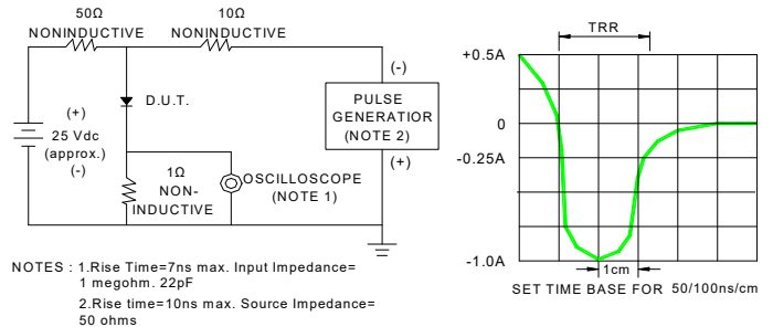
FIG.6-TEST CIRCUIT DIAGRAM AND FORWARD SURGE CURRENT
