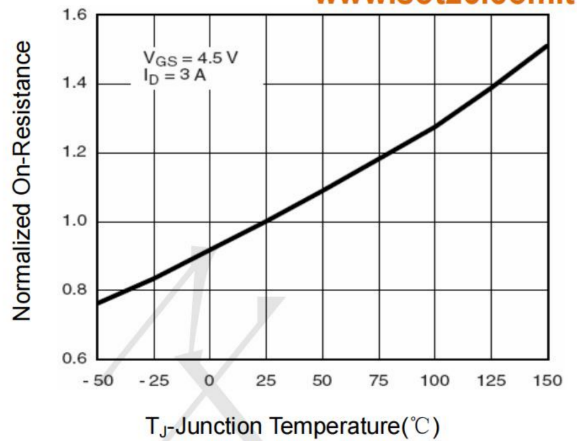
Figure 8 Drain-Source On-Resistance
