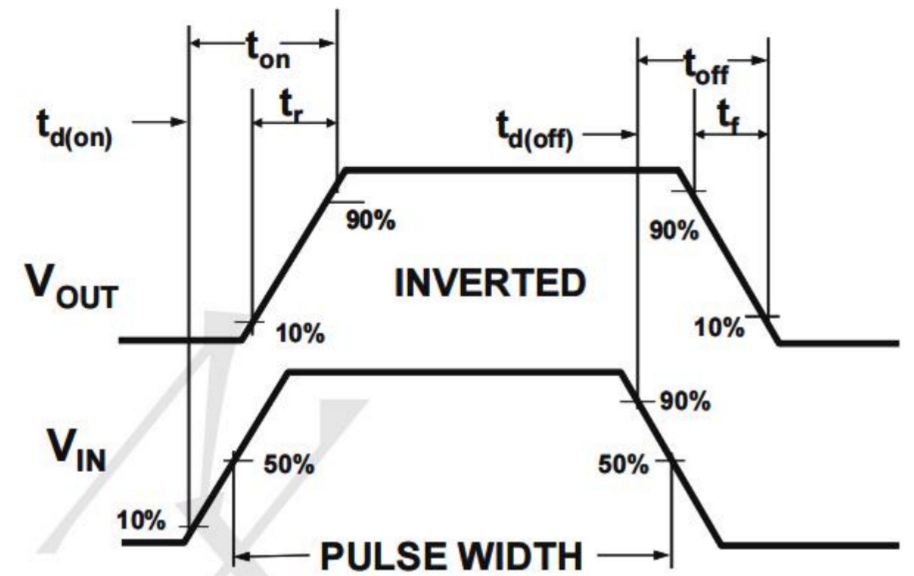
Figure 2: Switching Waveforms
